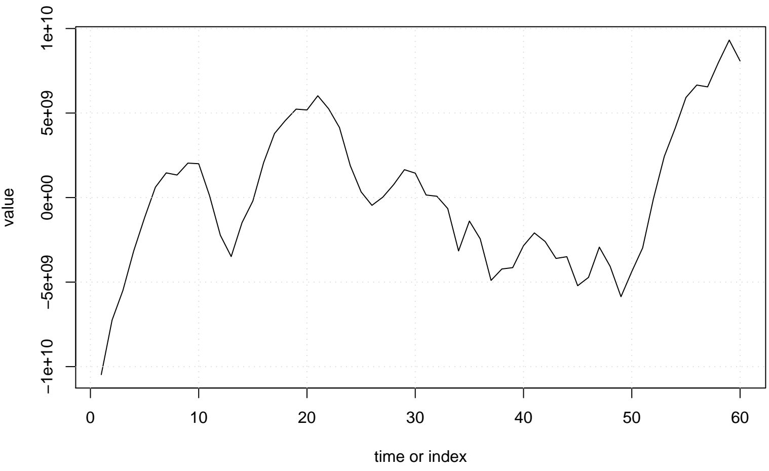
Run Sequence Plot of e[t]
