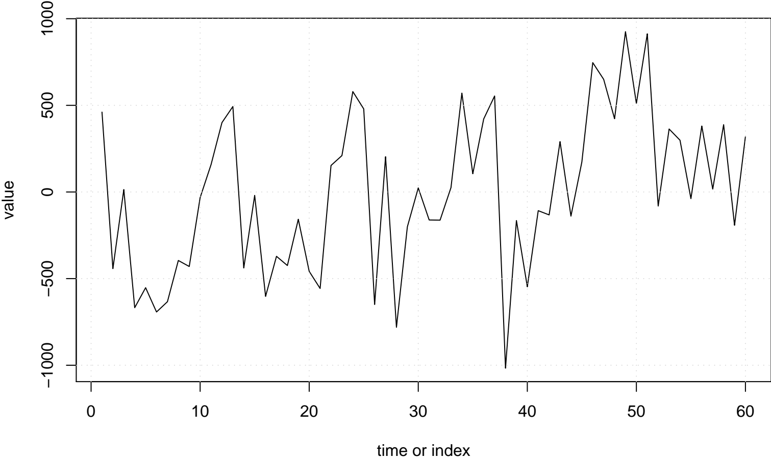
Run Sequence Plot of Y[t]
