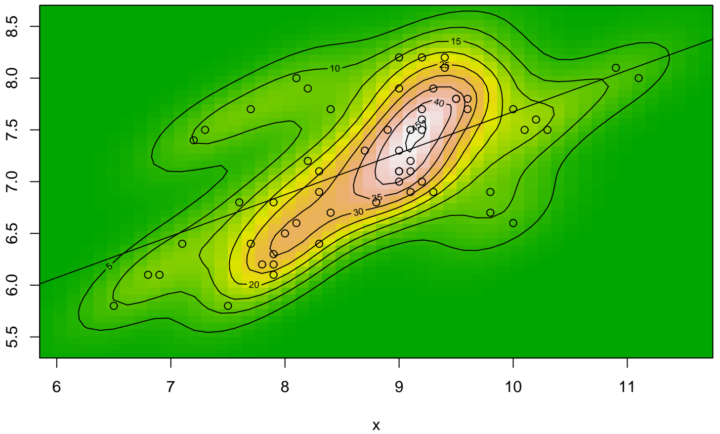
Bivariate Kernel Density
