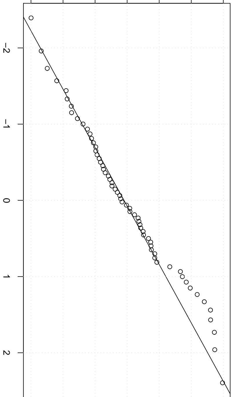
Theoretical Quantiles
