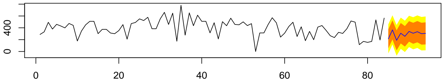
Forecasts from ARIMA(3,1,2)
