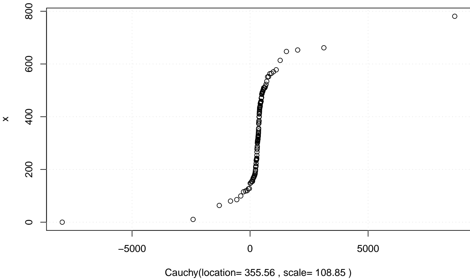
QQ plot (Cauchy)
