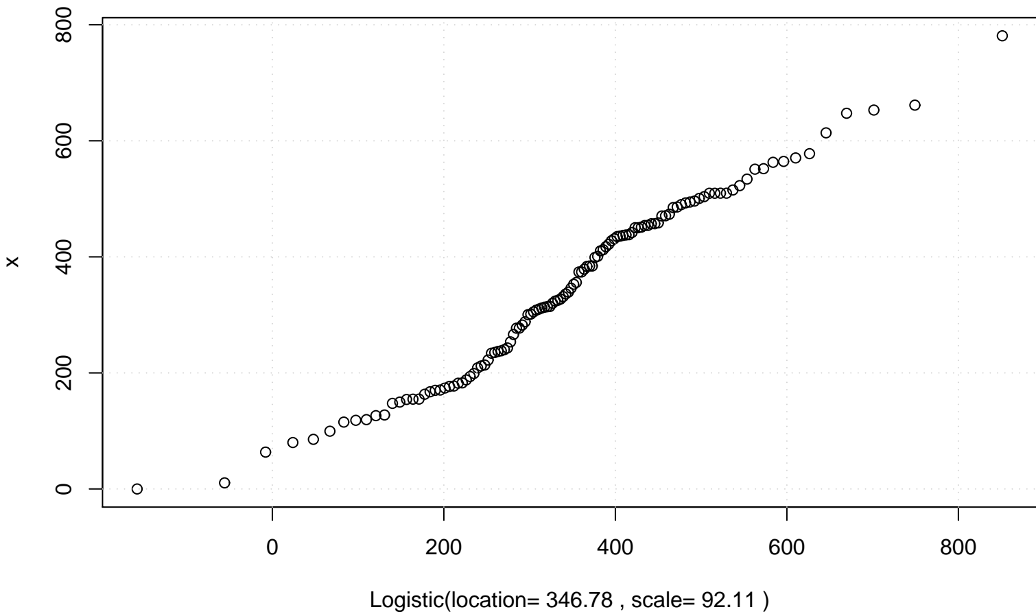
QQ plot (Logistic)
