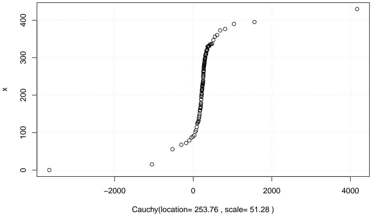
QQ plot (Cauchy)
