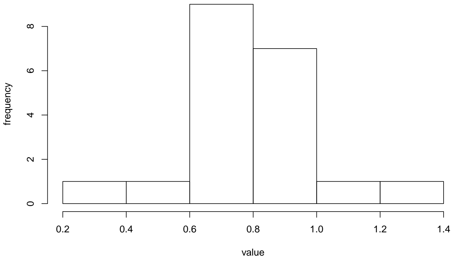
Histogram of MASE
