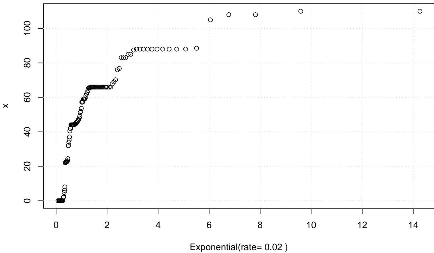
QQ plot (Exponential)
