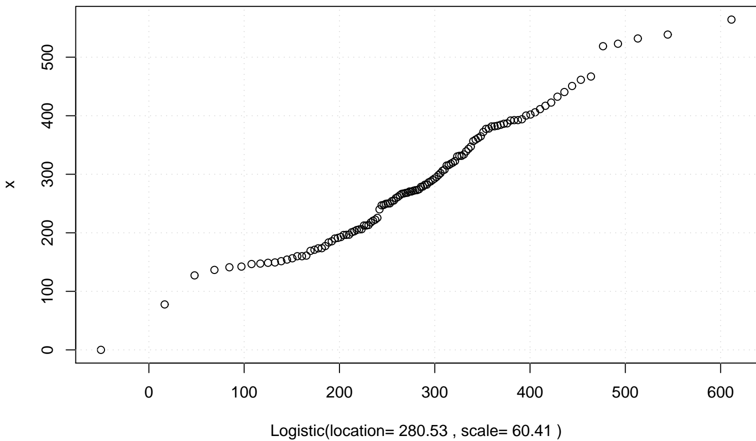
QQ plot (Logistic)
