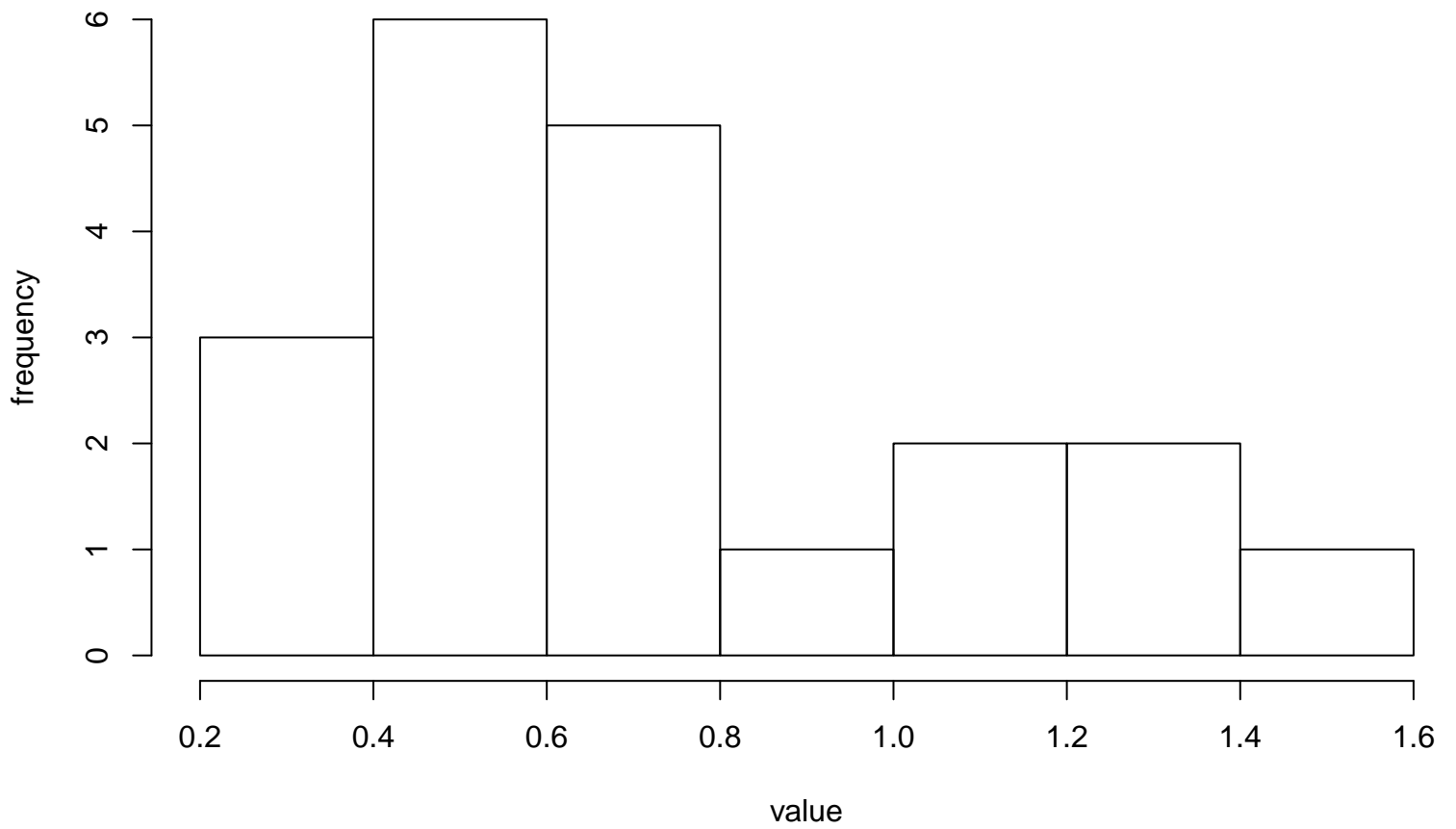
Histogram of MASE
