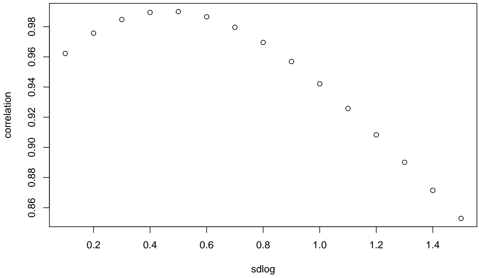
PPCC Plot – Lognormal
