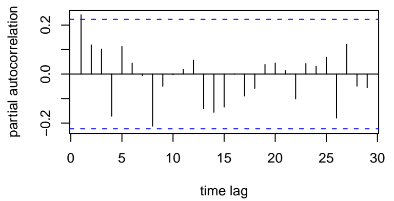
Residual PACF
