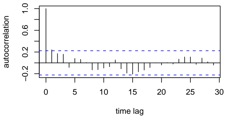
Residual ACF
