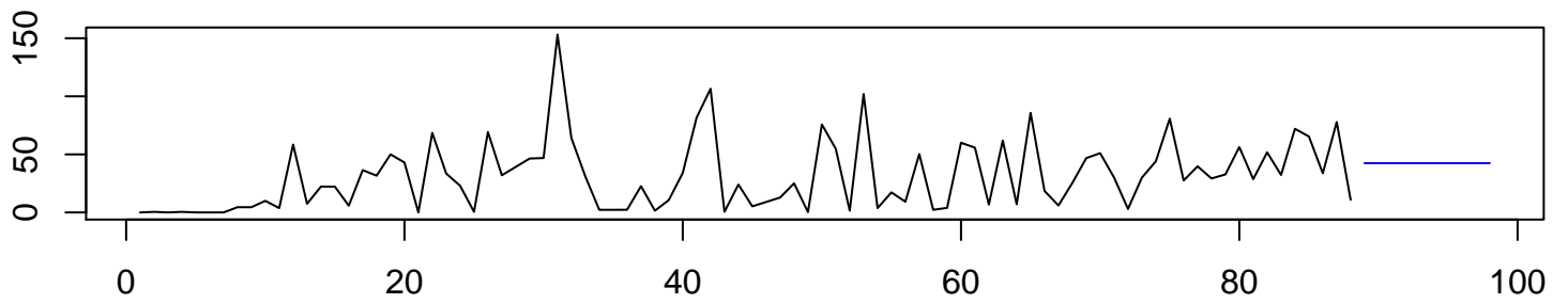
Forecasts from Croston's method
