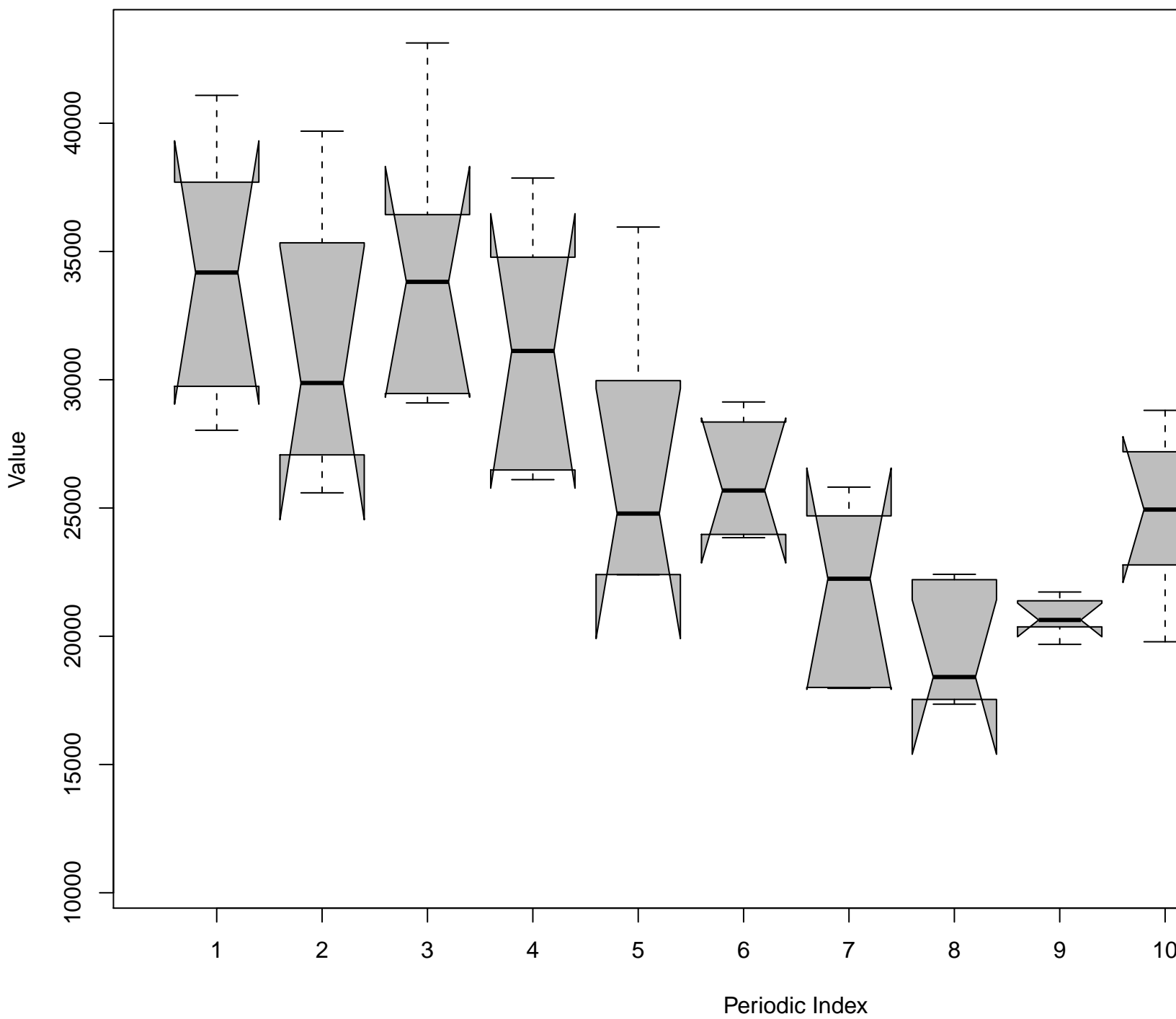
Notched Box Plots – Periodic Subseries
