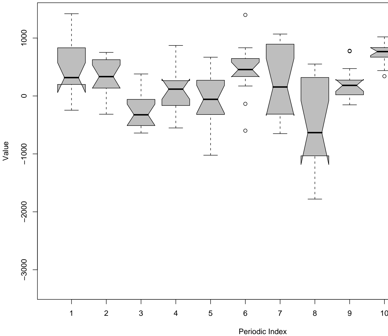
Notched Box Plots – Differenced Periodic Subseries
