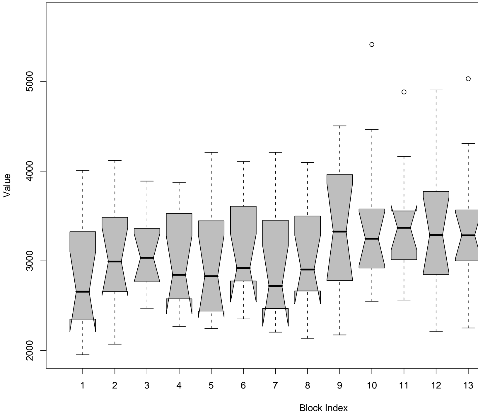
Notched Box Plots – Sequential Blocks
