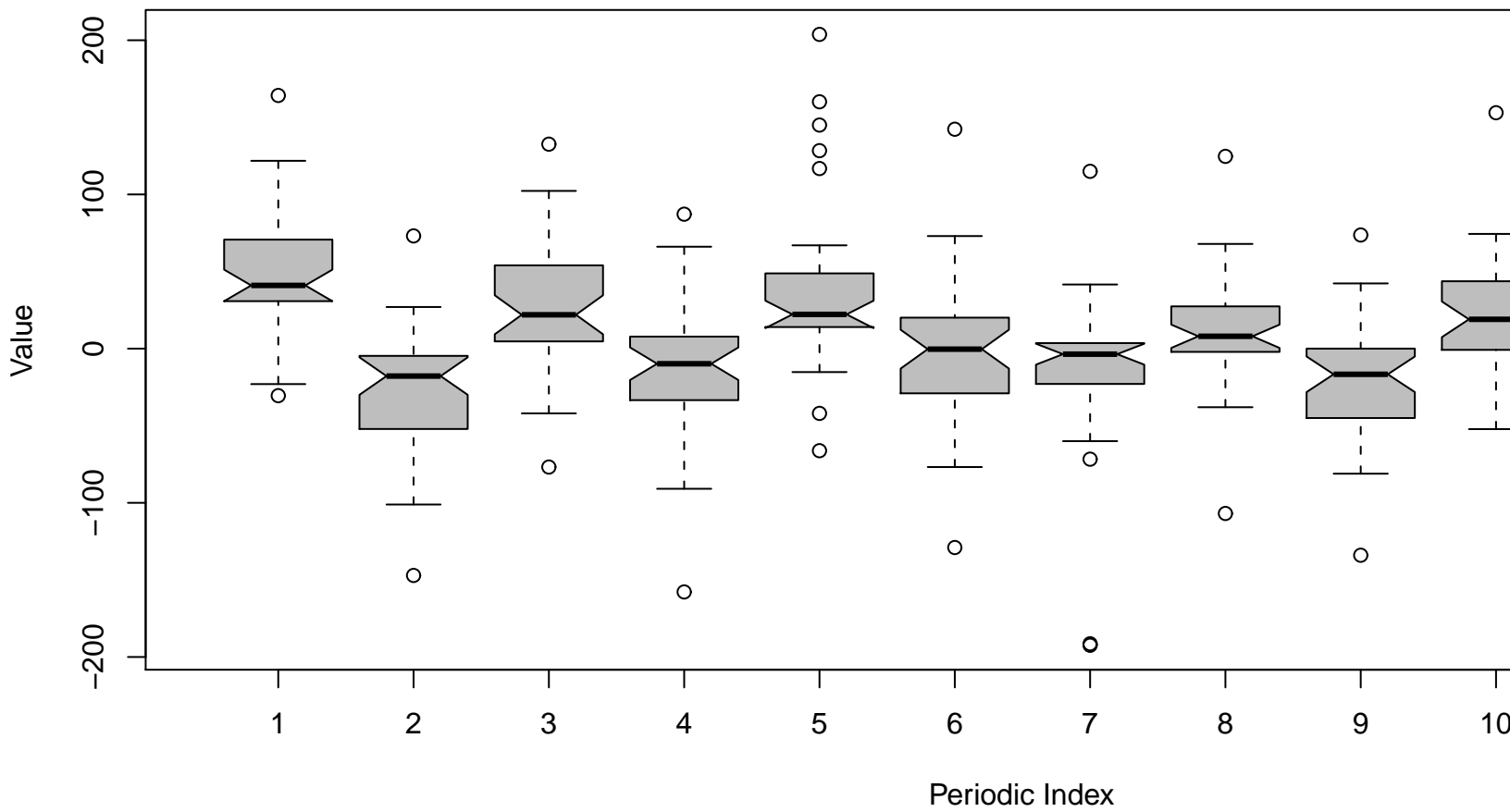
Notched Box Plots – Differenced Periodic Subseries
