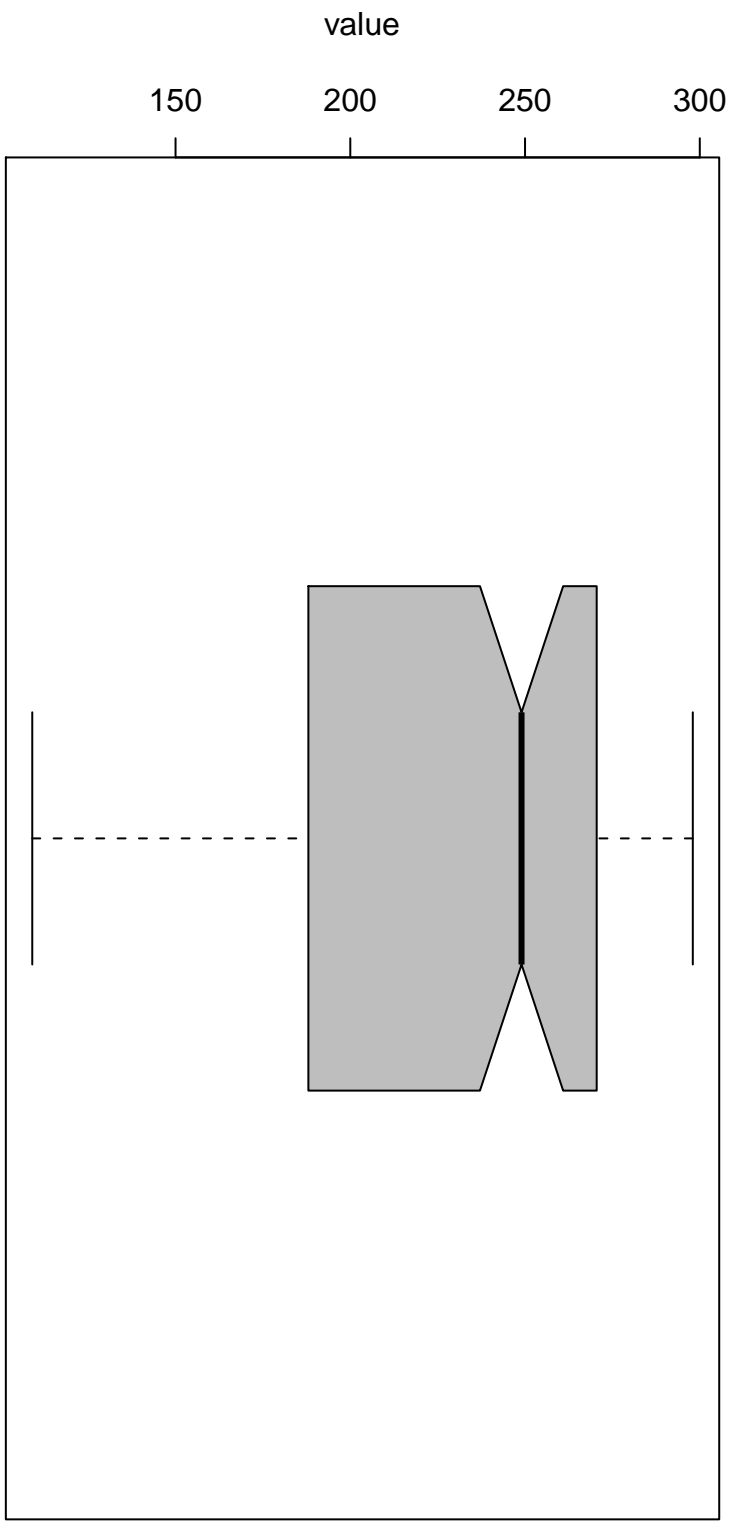
Notched Boxplots
