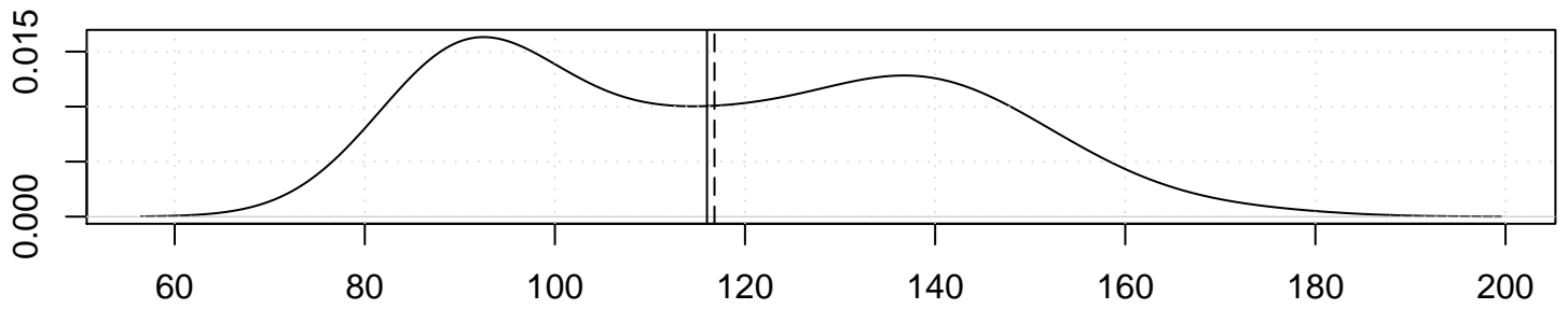
Density Plot – Gaussian Kernel
