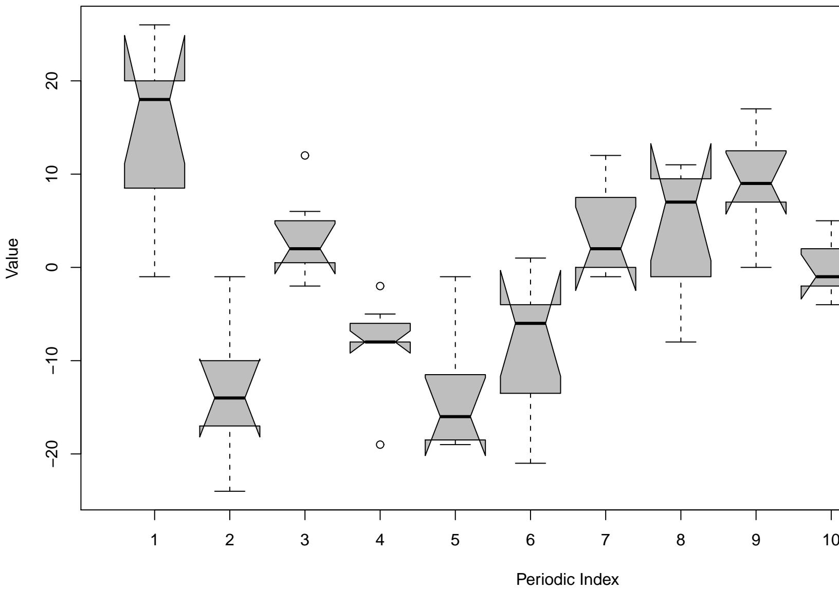
Notched Box Plots – Differenced Periodic Subseries
