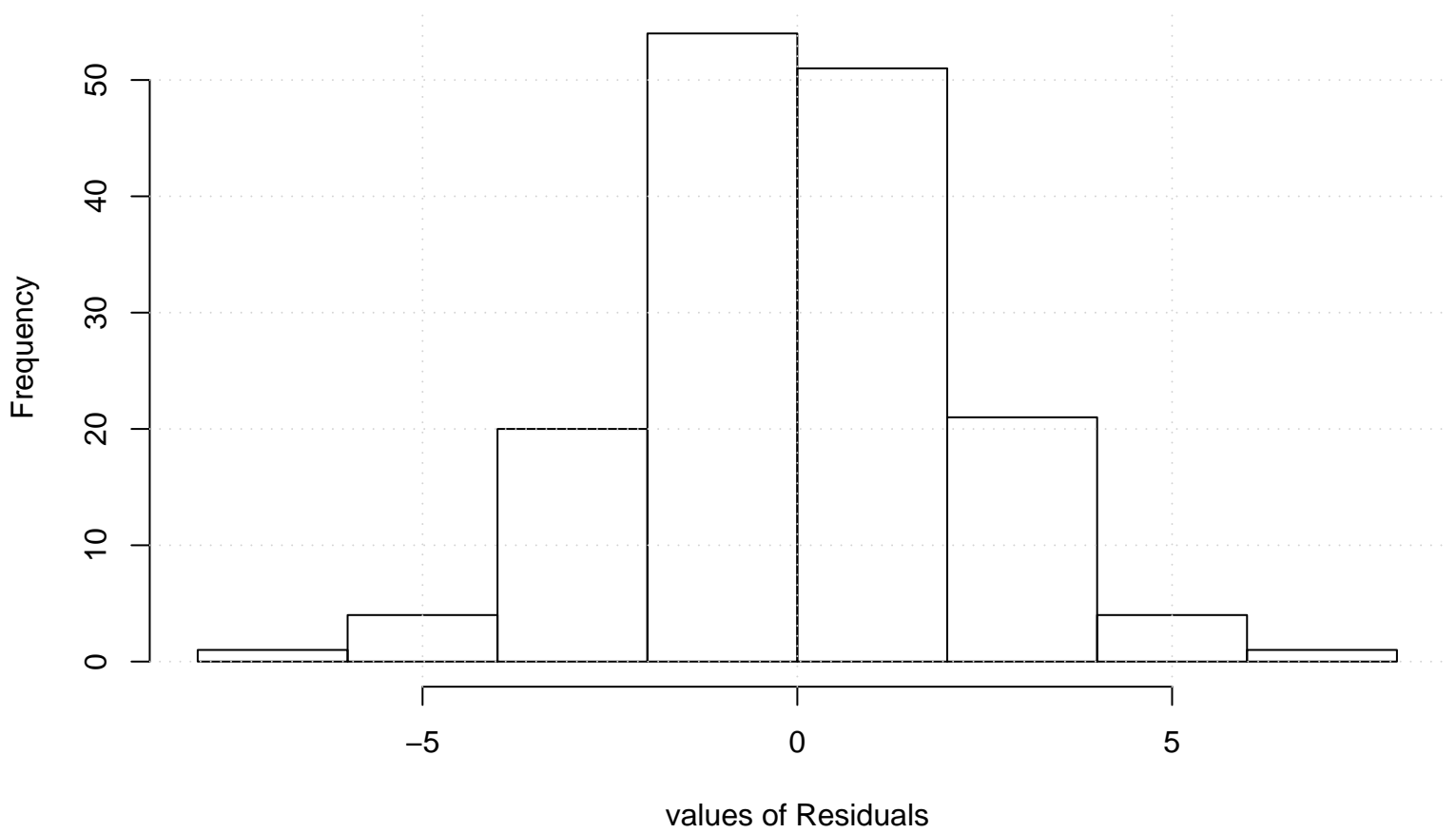
Residual Histogram
