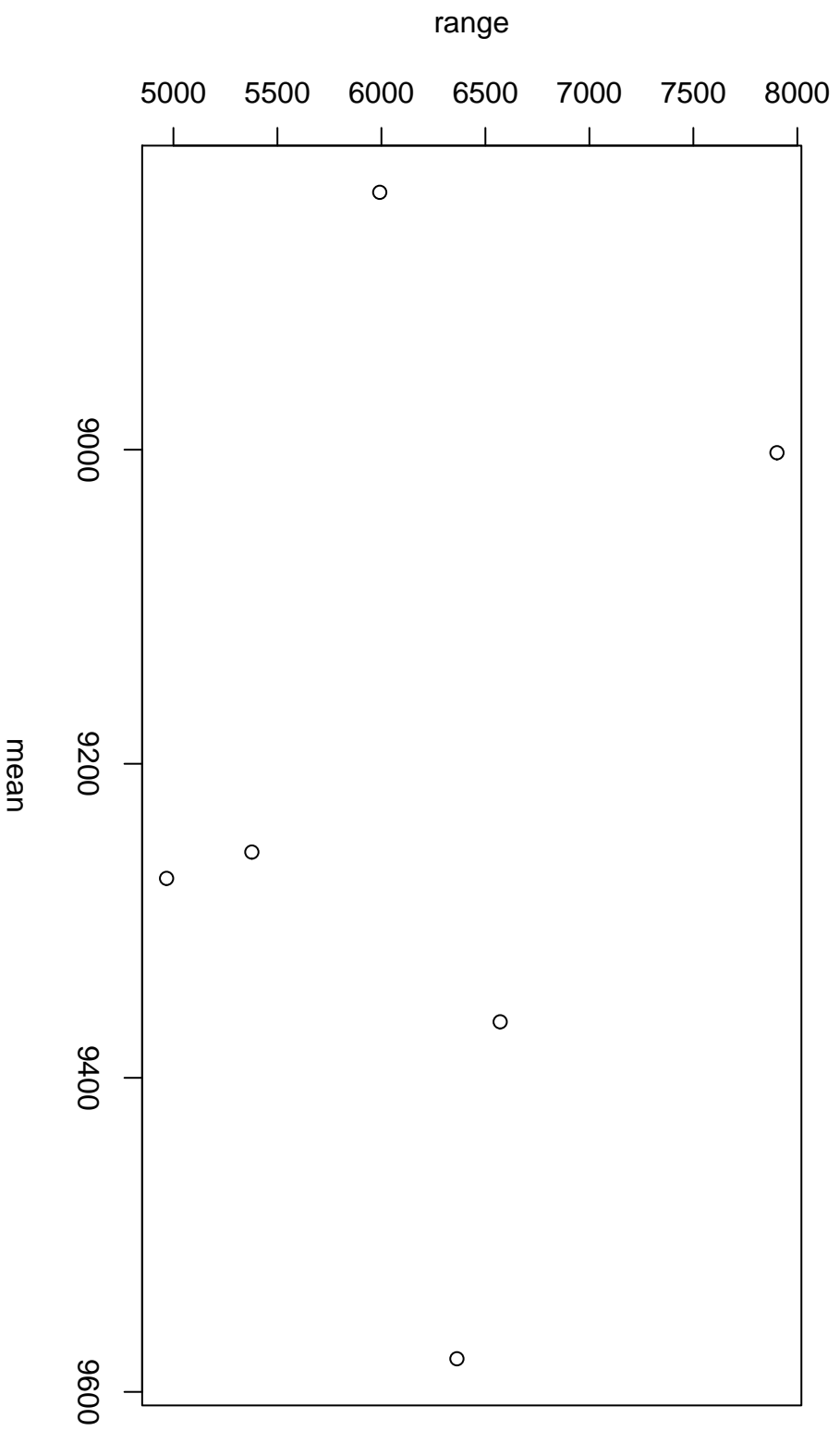
Range-Mean Plot
