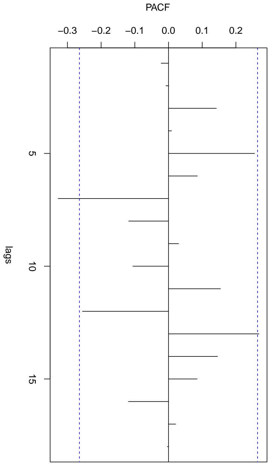
Partial Autocorrelation
