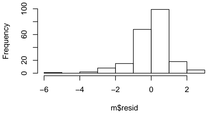
Residual Histogram
