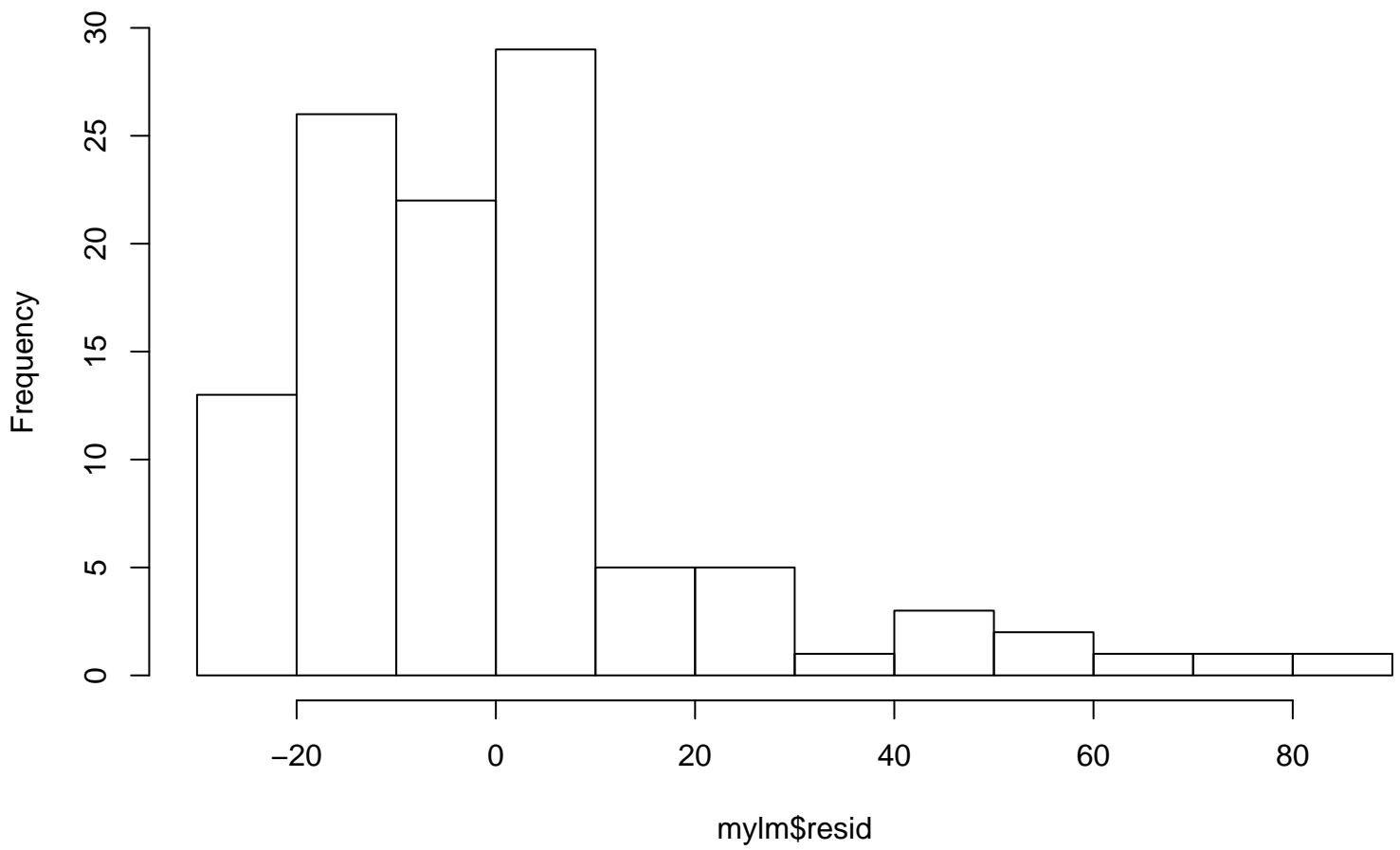
Histogram of e[t]
