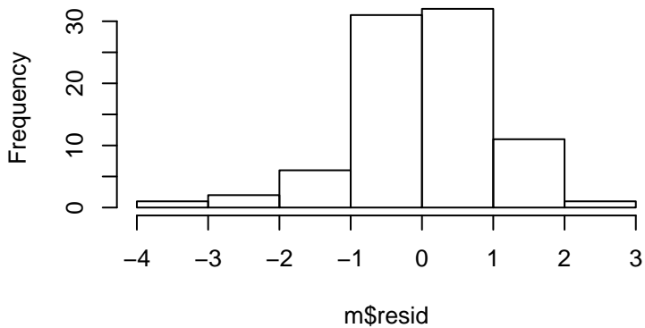
Residual Histogram
