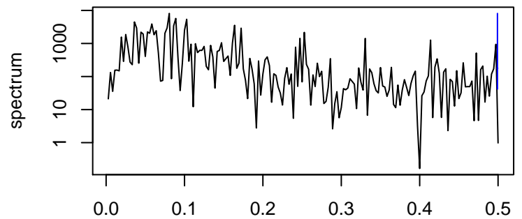
frequency bandwidth = 0.000802
