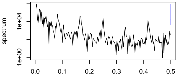
frequency bandwidth = 0.00077
