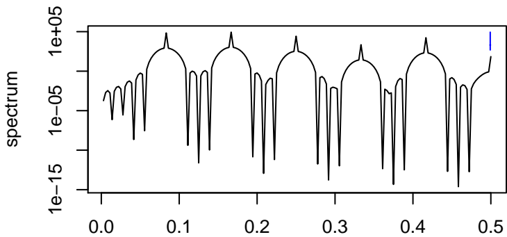
frequency bandwidth = 0.000802
