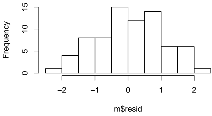
Residual Histogram
