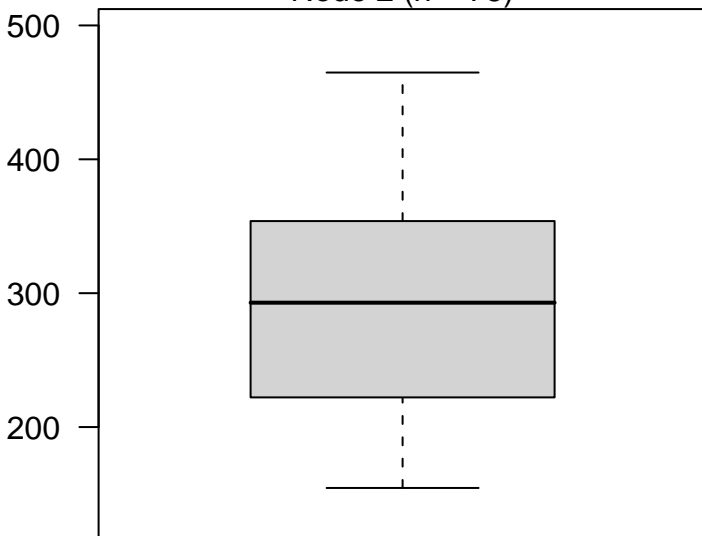
Node 2 (n = 75)
