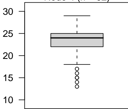
Node 4 (n = 92)
