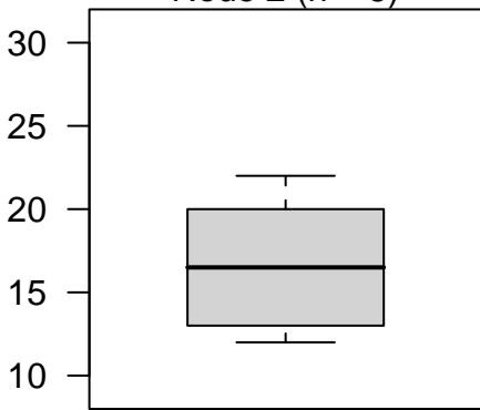
Node 2 (n = 8)
