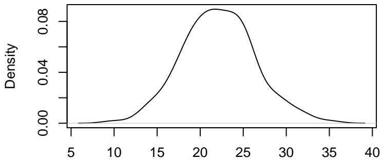
Kernel Density Plot of Actuals
