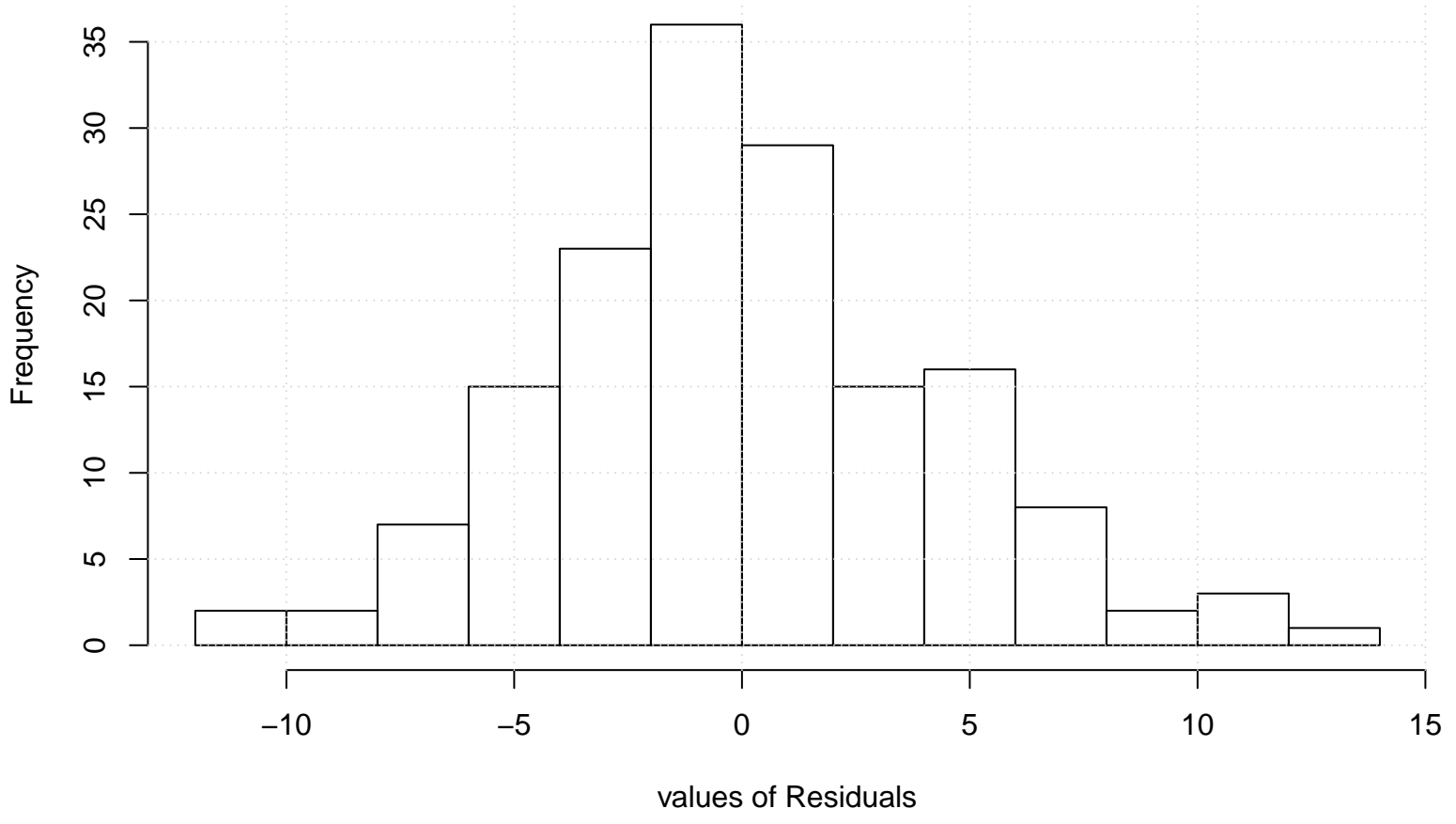
Residual Histogram
