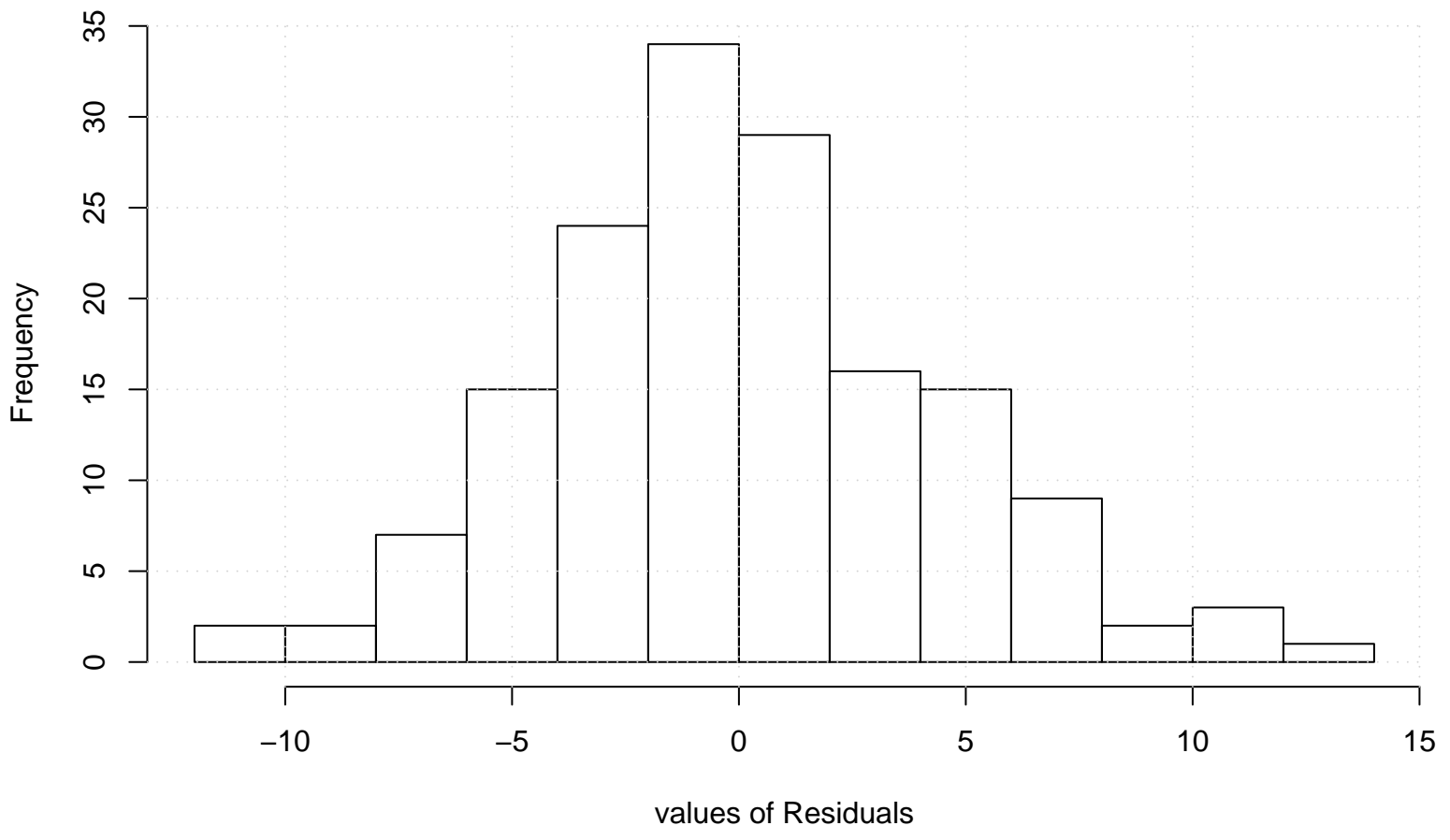
Residual Histogram
