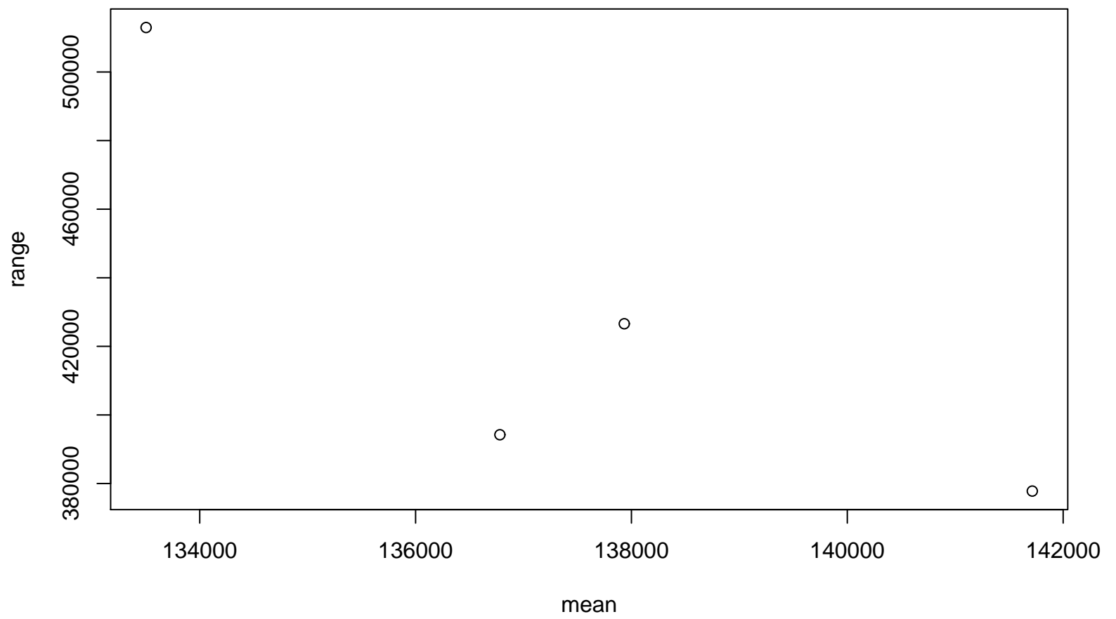
Range–Mean Plot
