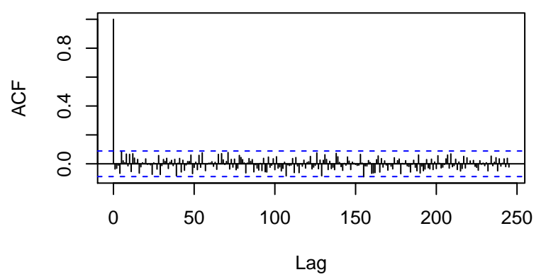
Standardized Residuals
