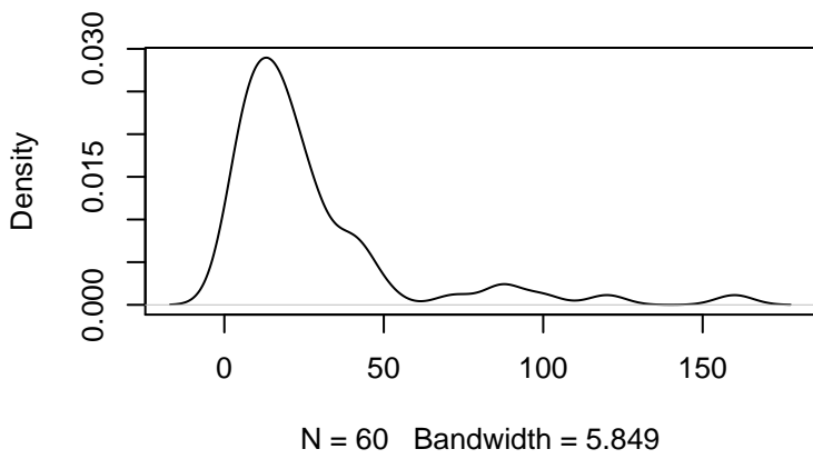
Kernel Density Plot of Actuals
