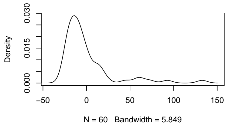
Kernel Density Plot of Residuals
