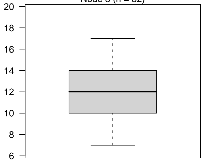
Node 3 (n = 32)
