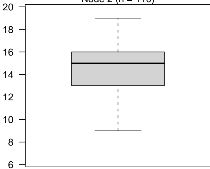
Node 2 (n = 110)
