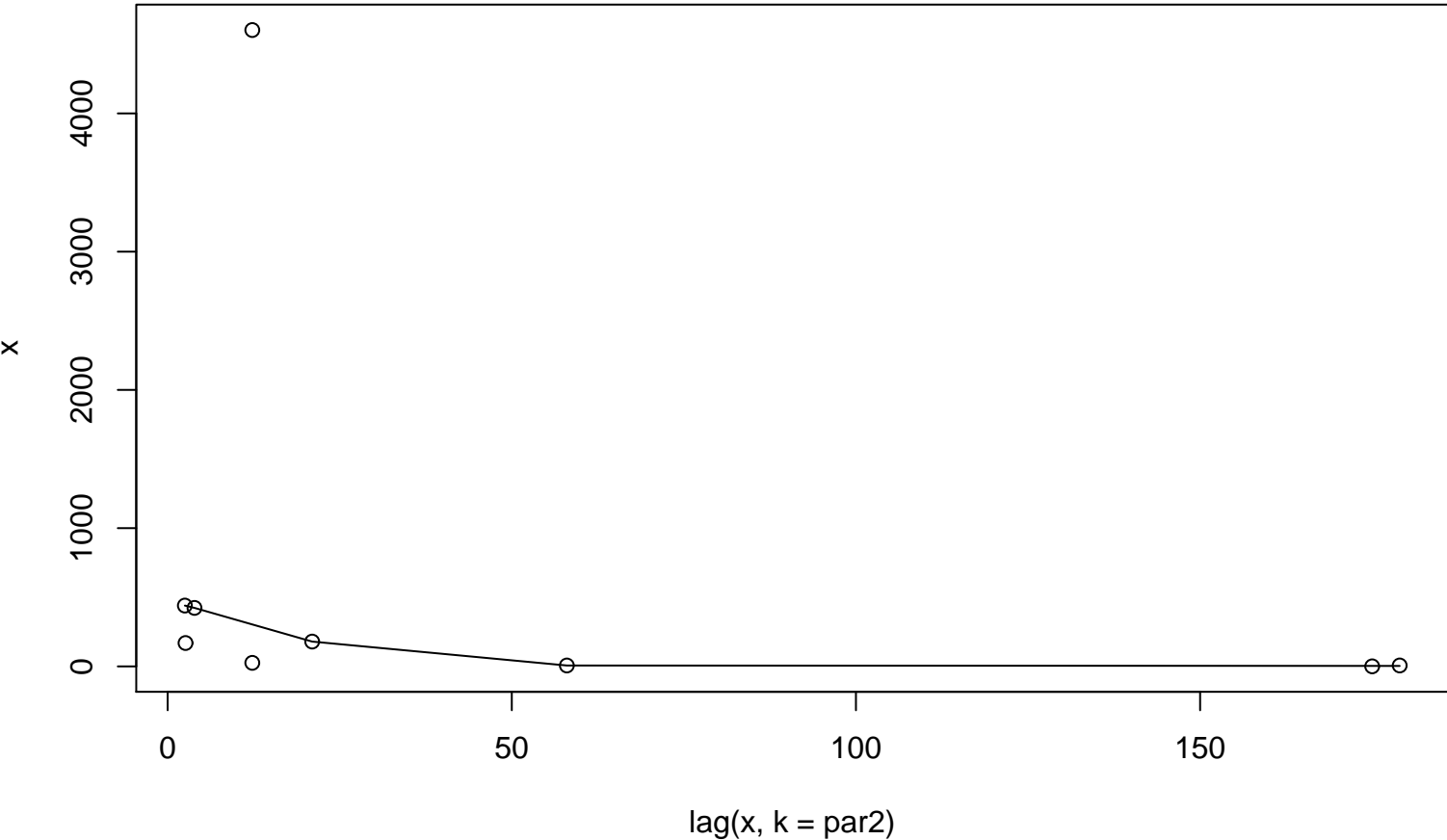
Lag plot (k=30), and lowess
