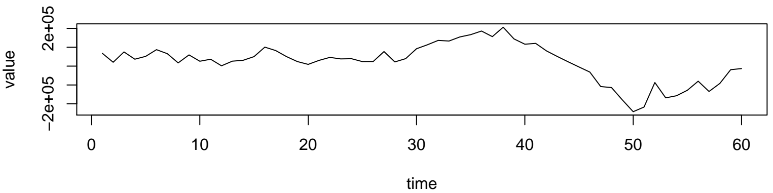
Working Time Series ( \lambda=1, d=0, D=1 )
