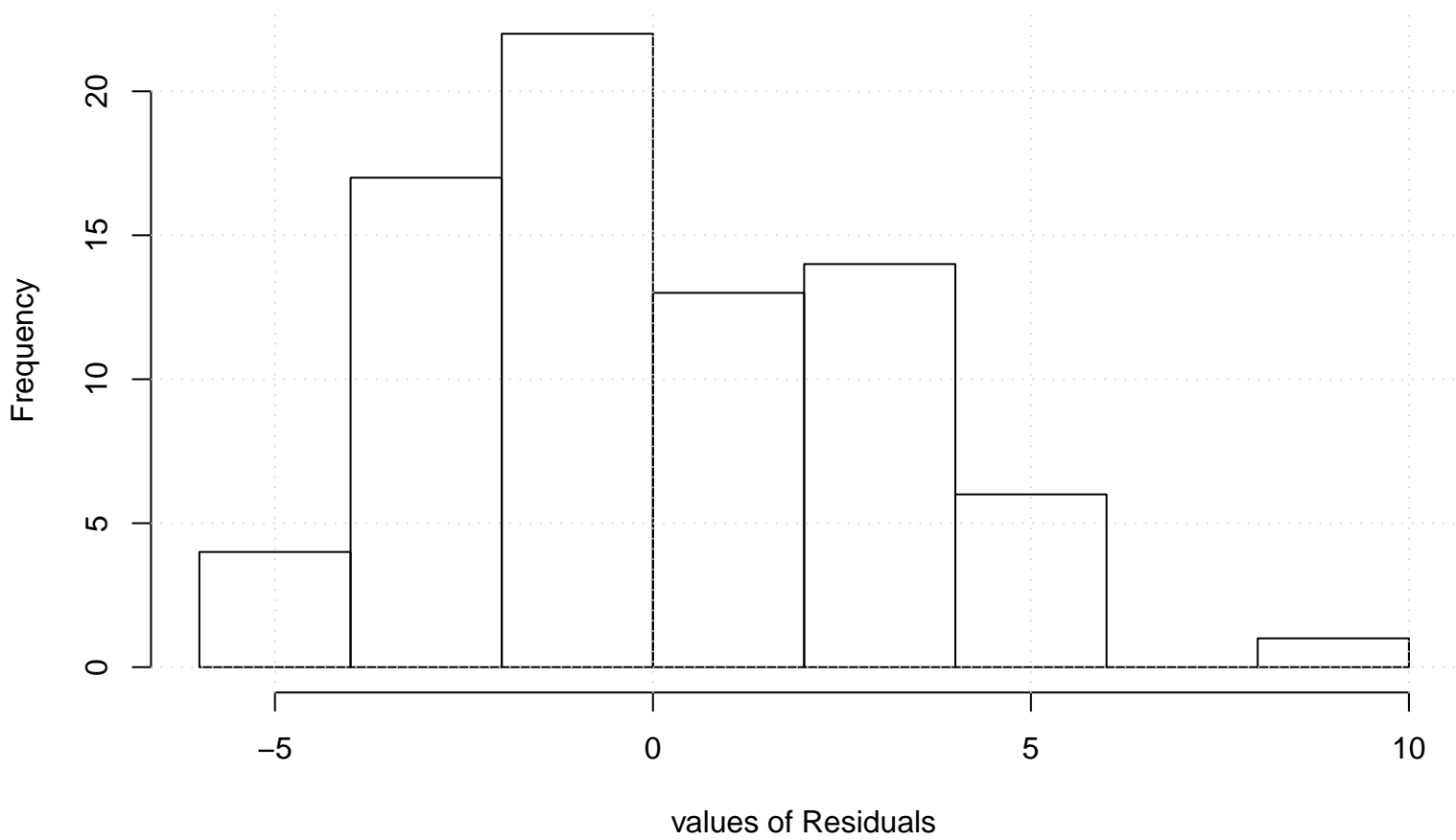
Residual Histogram
