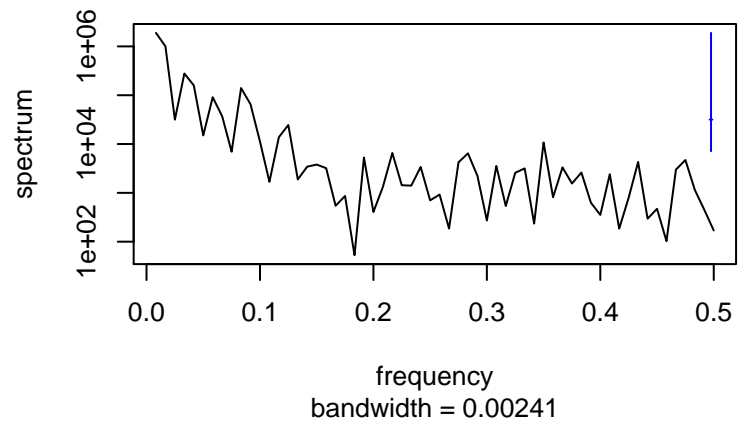
Standardized Residuals
