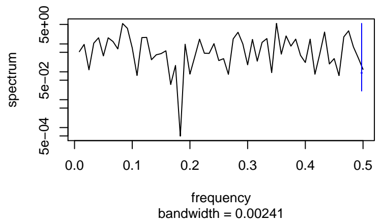
Standardized Residuals
