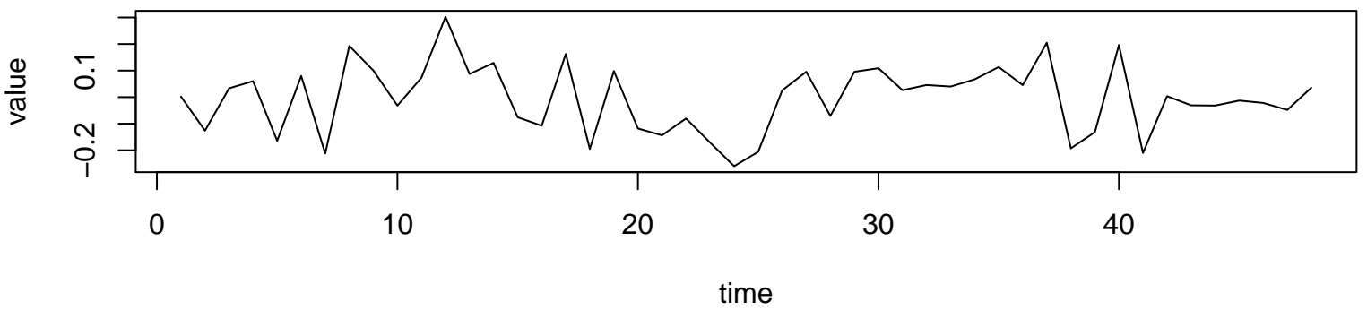
Working Time Series ( \lambda=0, d=0, D=2 )
