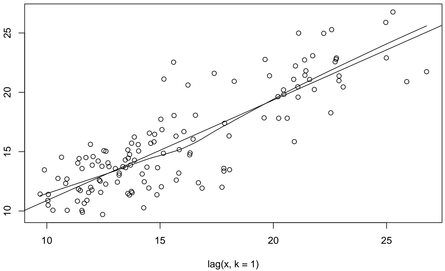
Lag plot (k=1), lowess, and regression line
