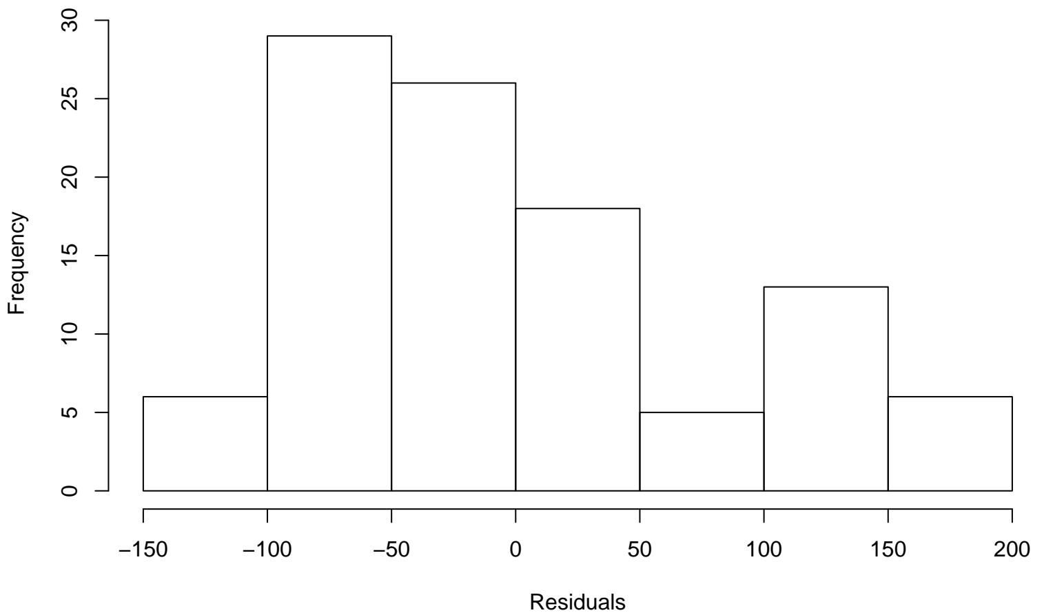
Residual Histogram
