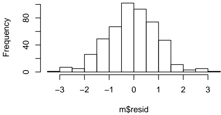
Residual Histogram
