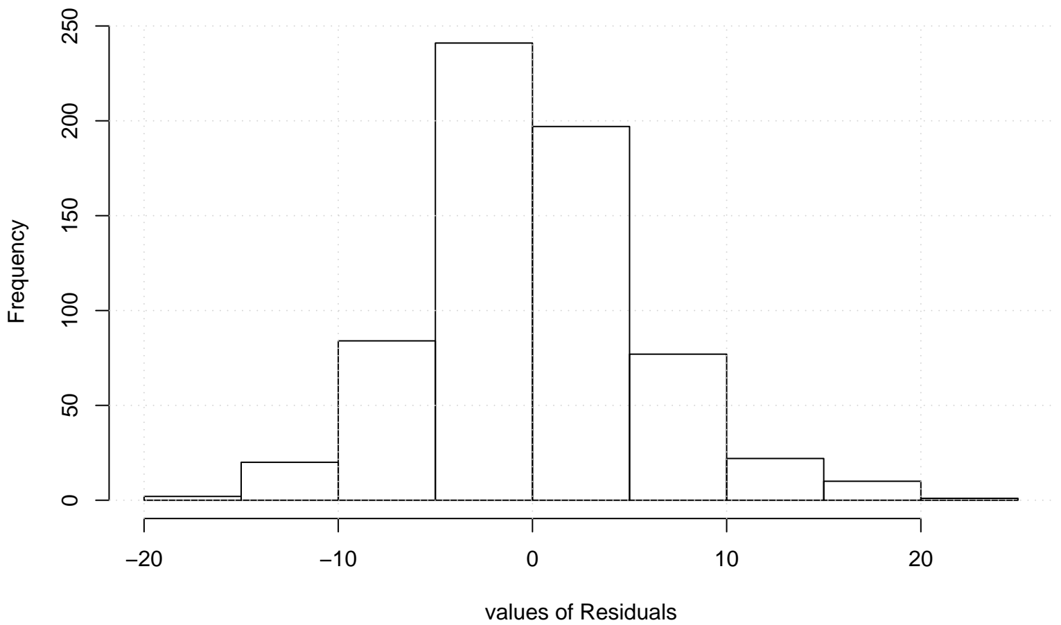
Residual Histogram
