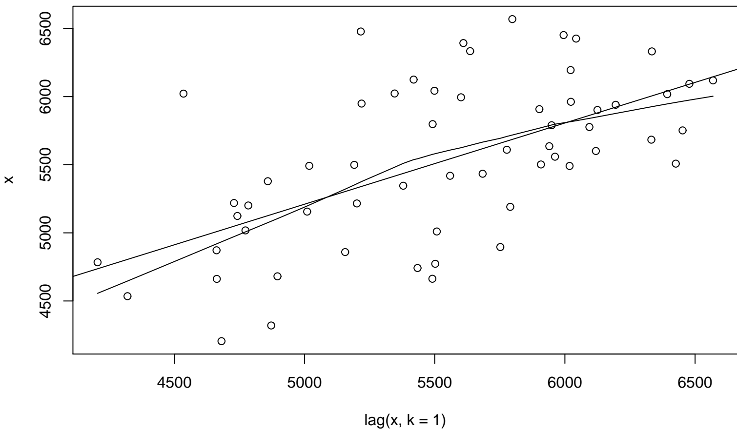
Lag plot (k=1), lowess, and regression line
