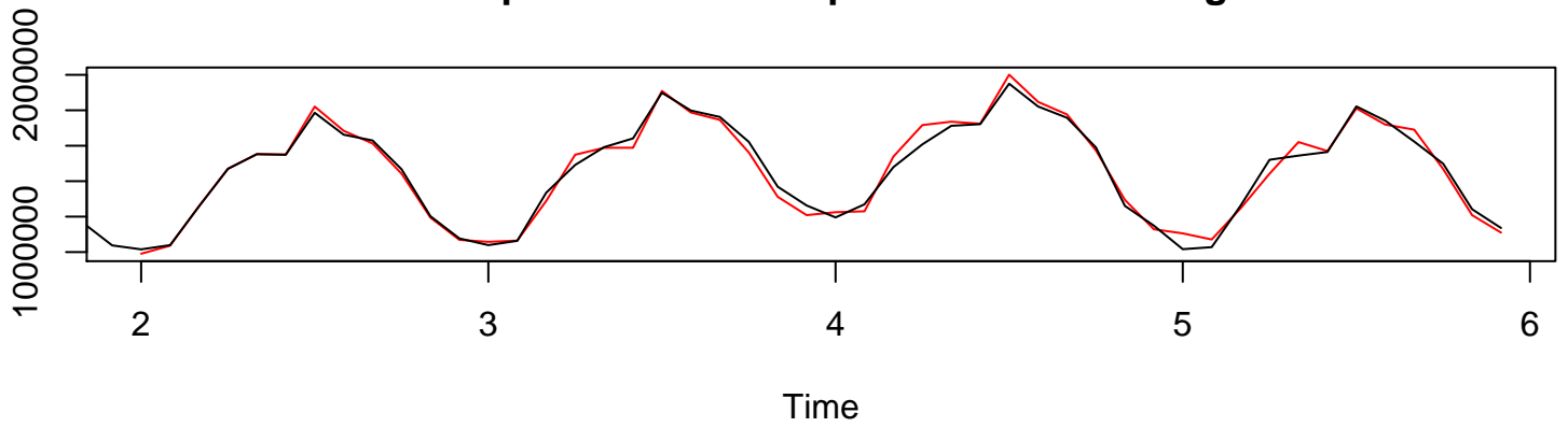
Interpolation Fit of Exponential Smoothing
